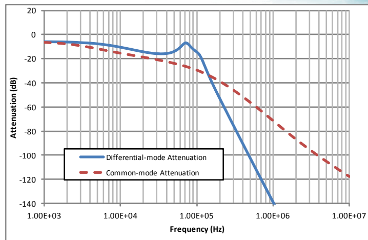
Figure 1: Typical Common Mode and Differential Mode Attenuation provided by the filter as a function of frequency when using parts suggested in the "Typical Connection Diagram". Source and load resistance are 50Ω.
