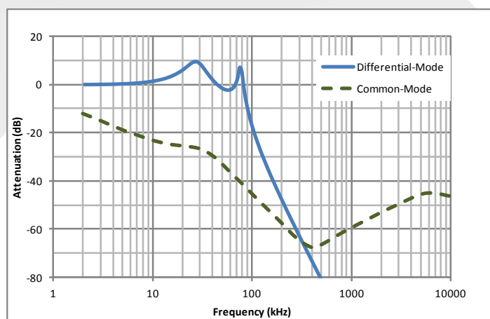
Figure A: Typical Common Mode and Differential Mode Attenuation as a function of frequency. 115 Vrms, 4.5 Arms. Source and load resistance are 50Ω.
