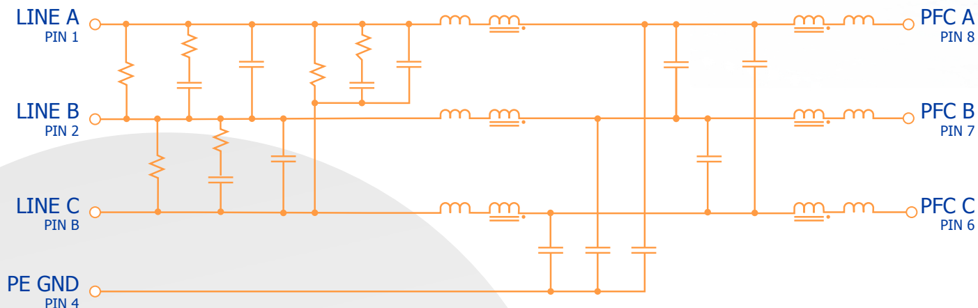
MACF-115-3PH-UNV-HT SynQor 3-Phase AC Line Filter
