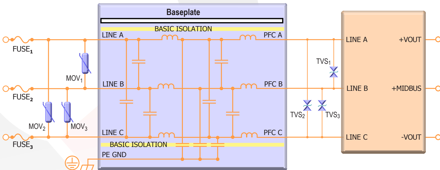
MACF-115-3PH-UNV-HT SynQor 3-Phase AC Line Filter
