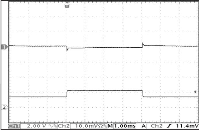
Figure 13: Output voltage response to step-change in load current 50%-75%-50% of I_{out} (max). Load capacitance: 1 \mu F ceramic and 10 \mu F 100 m \Omega ESR tantalum. Ch1: V_{out} (2 V/div). Ch 2: I_{out} (20 A/div).
