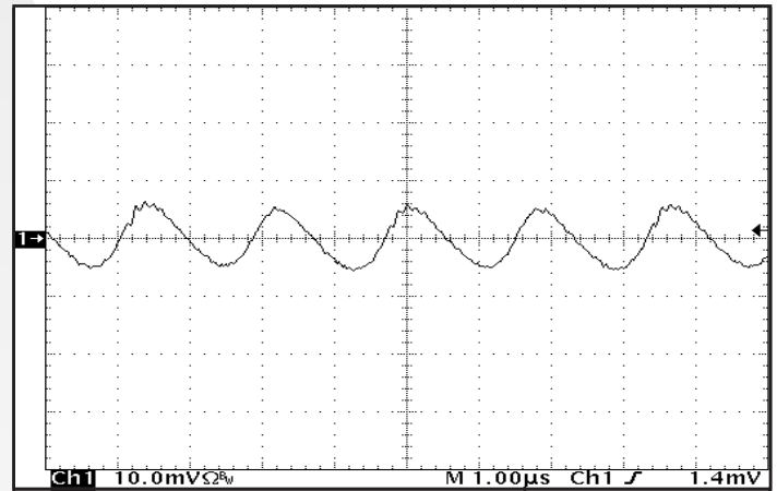
Figure 16: Input terminal ripple, i_c , at full load and nominal input voltage with 10 \mu H source impedance and 100 \mu F electrolytic capacitor (100 mA/div). Bandwidth: 20 MHz. See Figure 12.
