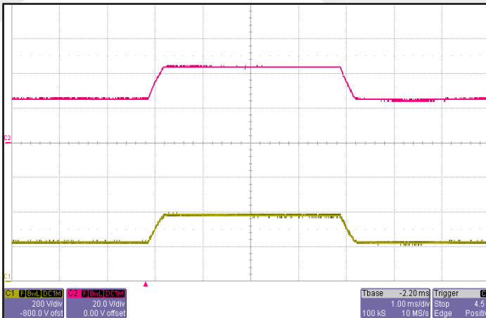
Figure 15: Output voltage response to step-change in input voltage 230 V-400 V-230 V in 250 \mu s. Load capacitance: 10 \mu F, 100 m \Omega ESR tantalum cap and 1 \mu F ceramic cap. Ch 1: V_{in} (200 V/div), Ch 2: V_{out} (20 V/div).
