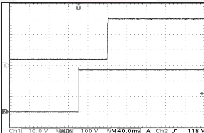
Figure 11: Turn-on transient at half resistive load and 100 \mu\text{F} output capacitance initiated by V_{in} . ENA previously enabled. Ch 1: V_{out} (10 V/div). Ch 2: V_{in} (100 V/div).
