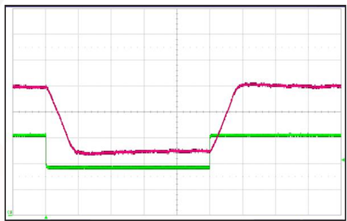
Figure 12: Characteristics of MCOTS HVNQ Family. MCOTS-N-28V-60-HG shown Output Current vs Iset pin voltage dynamics; 28Vin 10Vout (5uS/div). Top Trace: Output Current (2A/div). Bottom Trace: Iset pin voltage (200mV/div).
