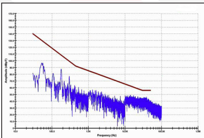
Figure 5: MIL-STD-461E Method RE101 Low Frequency Radiated Emissions of the MQME-270-P filter with a MQFL-270-05S at 120W output. Limit line (in brown) is the 'Standard Curve' from MIL-STD-461C Method RE01, which is more strict than all RE101 limits.
