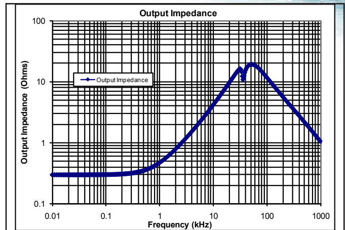
Figure 2: Calculated Output Impedance (magnitude) of the filter looking back into its output pins with the input pins connected to a source with zero source impedance assuming no other parasitic coupling in the system.
