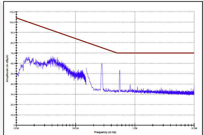
Figure 4: MIL-STD-461E Method CE102 High Frequency Conducted Emissions of the MQME-270-P filter with a MQFL-270-05S at 120W output. Limit line (in brown) is the 'Basic Curve'.
