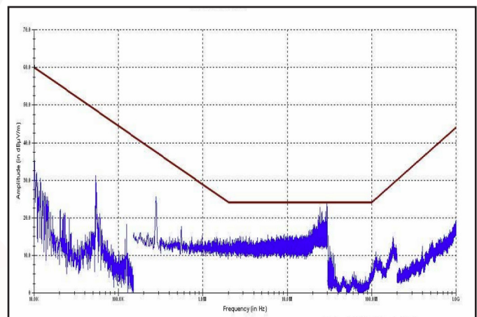
Figure 6: MIL-STD-461E Method RE102 High Frequency Radiated Emissions of the MQME-270-P filter with a MQFL-270-05S at 120W output. Limit line (in brown) is the 'Submarine External to Pressure Hull Curve'.
