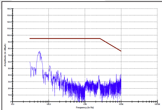
Figure 3: MIL-STD-461E Method CE101 Low Frequency Conducted Emissions of the MQME-270-P filter with a MQFL-270-05S at 120W output. Limit line (in brown) is the 'Submarine Applications DC Curve'.
