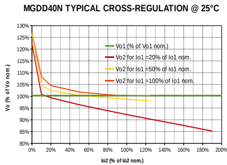
Vo2 regulation versus current Io2 as % of nominal Io2nom @ V01 various fixed load as a % of nominal current Io1nom
