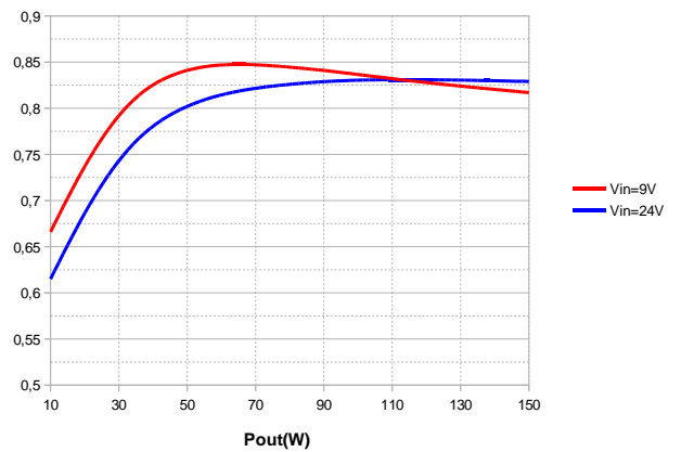
MGDS-150-H-J - Efficiency vs Output Power
