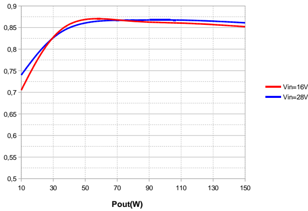
MGDS-150-O-I - Efficiency vs Output Power
