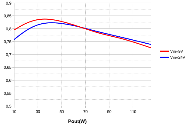
MGDS-150-H-C - Efficiency vs Output Power
