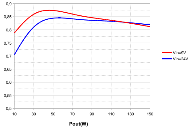
MGDS-150-H-F - Efficiency vs Output Power
